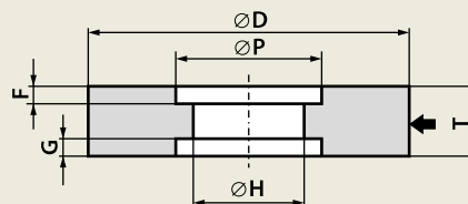
7 profile - D x T x H - P...F...G...
