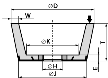
Taper cup wheel with a central threaded insert 1113 - D / J × T × H - W...E...K...
