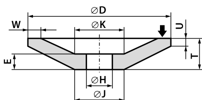
Dish wheel 12 - D / J × T / U × H - W...E...K...
