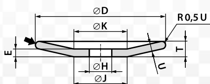
Saucer wheel 13 - D / J × T / U × H - E...K...
