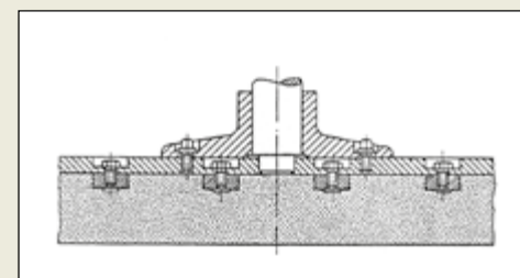
Fig. Grinding wheel bolted to a backplate and bolted to the machine spindle.
