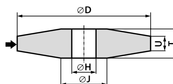
Wheel tapered on both sides 4 - D / J × T / U × H
