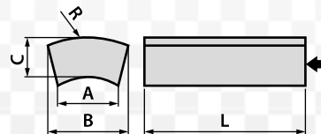
Segment, with inner and outer radius 3104 - B / A × C × L - R...
