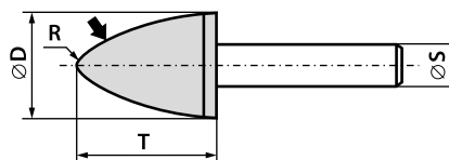
Mounted point, ogival shape 5220 - D × T × S - R...
