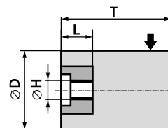
Cones and plugs, cylindrical 18 - D × T - H × L
