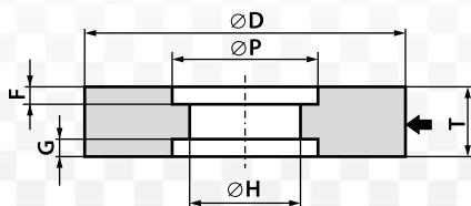
Wheel recessed on both sides 7 Profile* - D \times T \times H - P \dots F \dots G \dots
