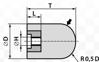
Cones and plugs, roll shaped with a threaded insert 18R - D × T - H × L
