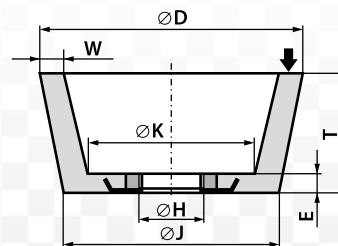
Taper cup wheel with a central threaded insert 1112 - D / J \times T \times H - W \dots E \dots K \dots
