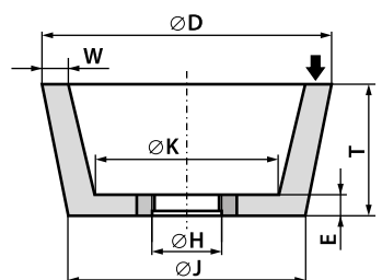
Taper cup wheel with a central threaded insert 1114 - D / J × T × H - W...E...K...
