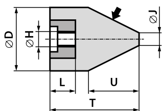
Cones and plugs, cylinder-conical with a threaded insert 19 - D / J \times T / U - H \times L
